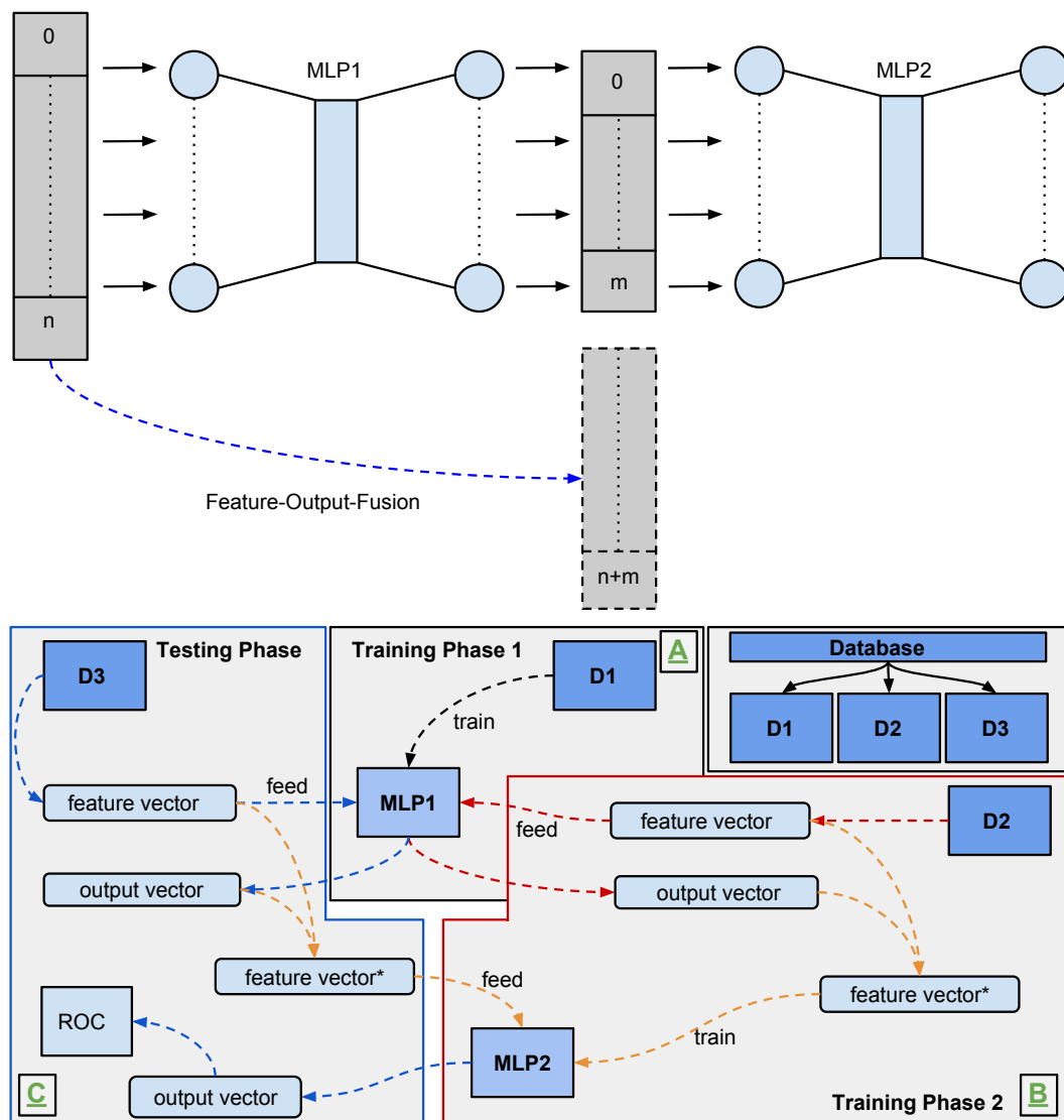
Figure 13. A sketch of our two-stage MLP model ( top ) and an affiliated training procedure ( bottom ). For an input histogram of size n = 625 and an output layer size of m = 10 neurons, the secondary MLP receives the primary MLPs' output activation plus another histogram as input. In our training procedure, we split our dataset D in three parts D_1 , D_2 and D_3 , such that we may train our two MLPs on independent parts of the dataset and test it on unseen data.
