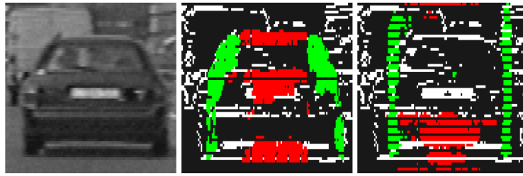
Fig. 5. Hausdorff distance classifier: each region is compared with two models.
