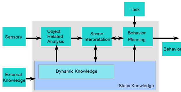
Fig. 16. Architecture for a driver assistance system.
