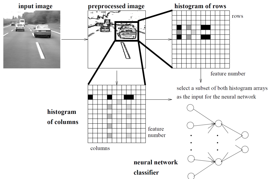
Fig. 4. The LOC-classifier process.
