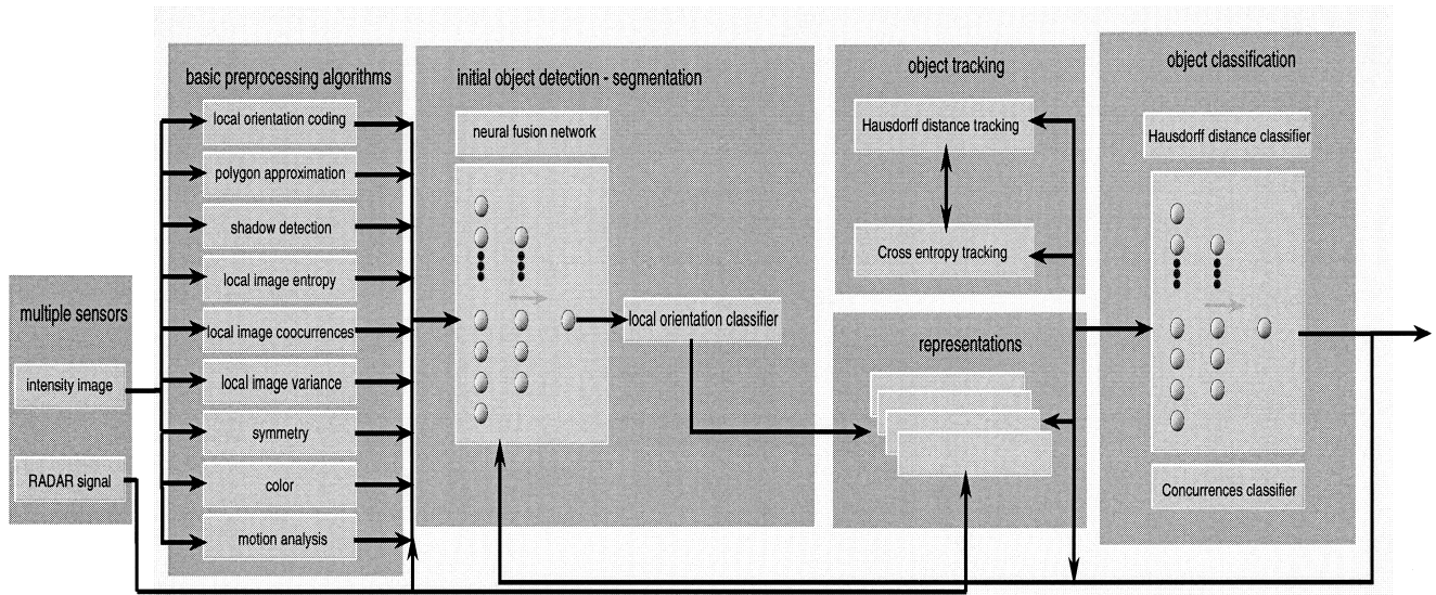
Fig. 10. Sensor information processing. In the preprocessing part an extraction of relevant features from multiple sensors is done. In the segmentation part a detection of initial object hypotheses is realized. In the object tracking and classification parts a verification of the hypotheses are performed. In the sensor-based representations task-dependent saliency maps are implemented to verify the output of the segmentation, the classification and the tracking part of the system.
